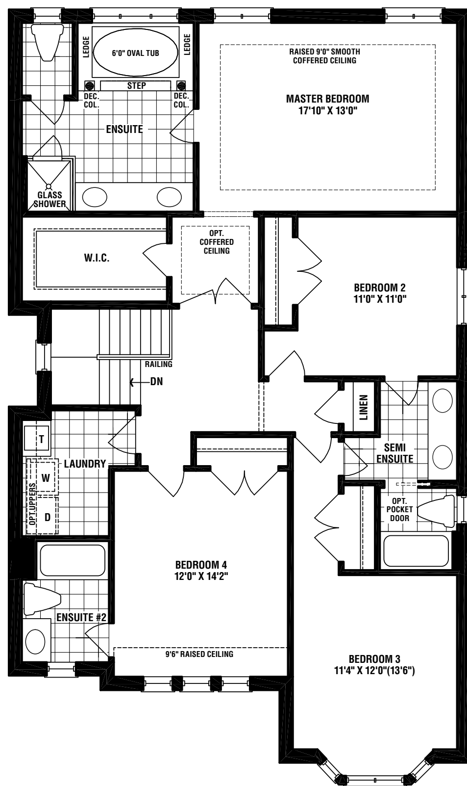
SECOND FLOOR ELEV. 'A'
