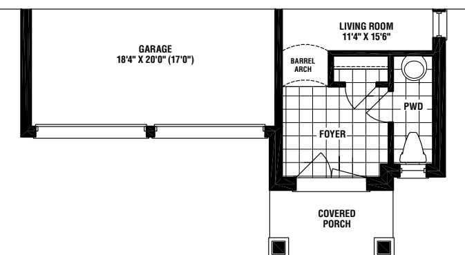
PART. GROUND FLOOR ELEV. 'C'
