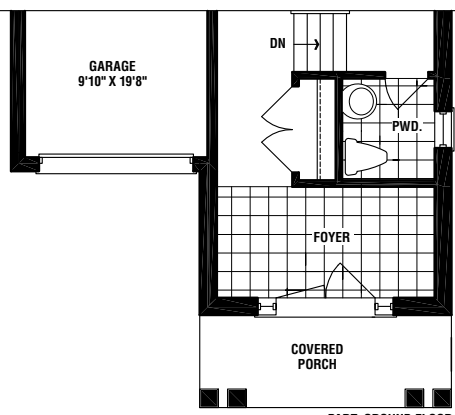
PART. GROUND FLOOR ELEV. 'B'
