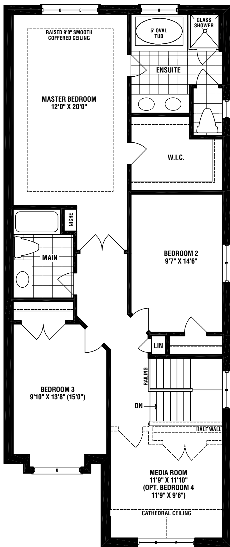
SECOND FLOOR ELEV. 'A'
