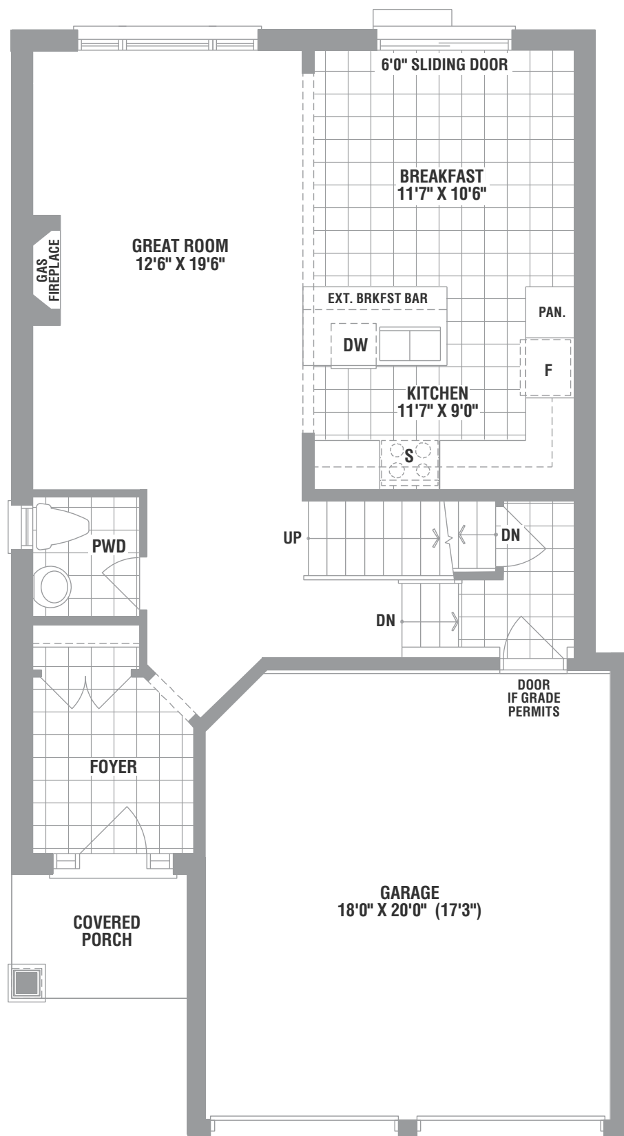
GROUND FLOOR ELEV. 'A', 'B' & 'C'
