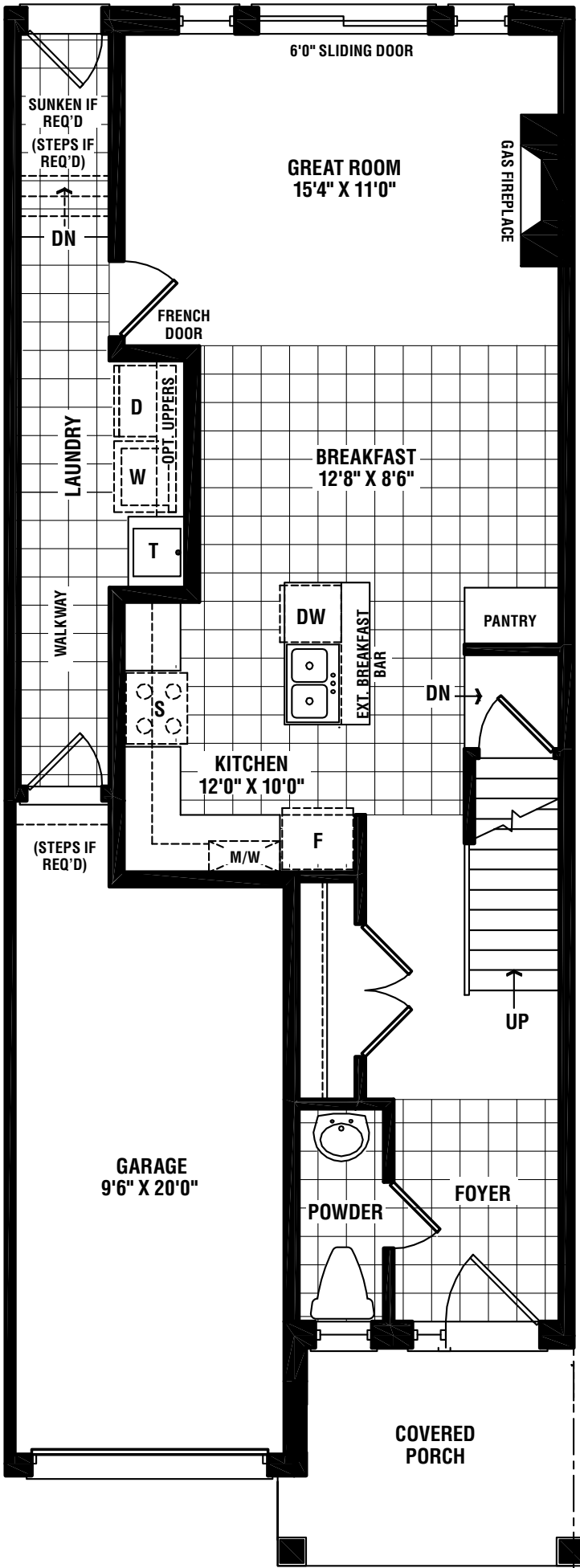
GROUND FLOOR ELEV. 'A'
