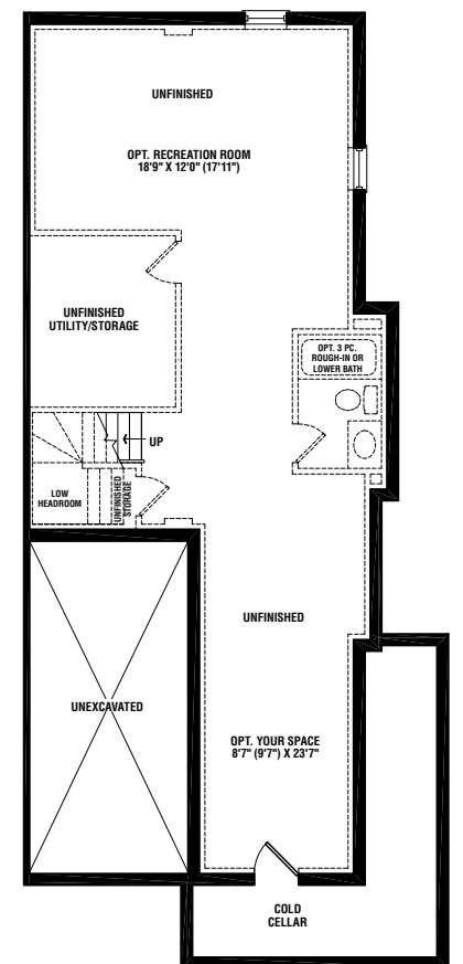
LOWER LEVEL ELEV. 'B'
