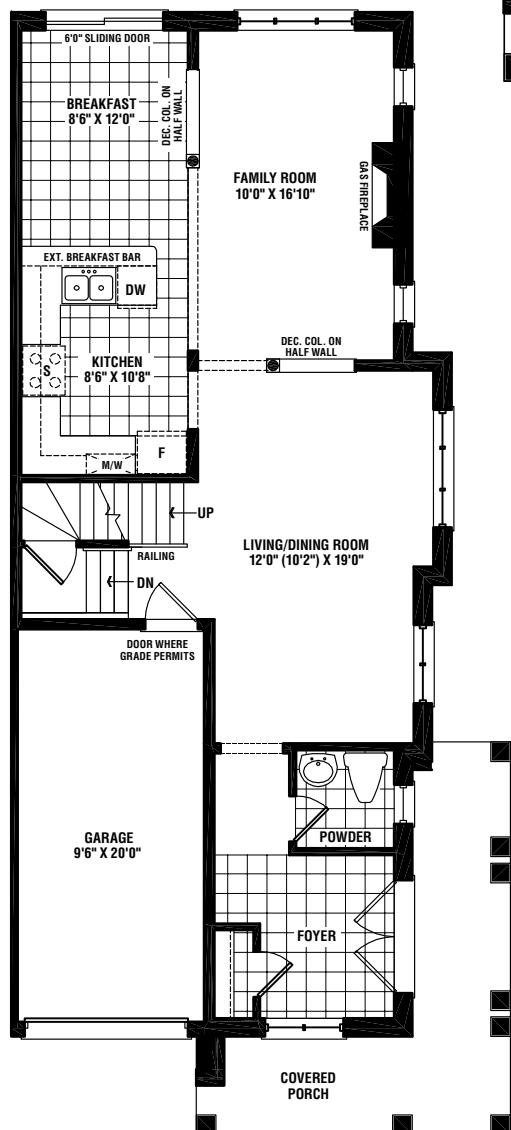
GROUND FLOOR ELEV. 'B'
