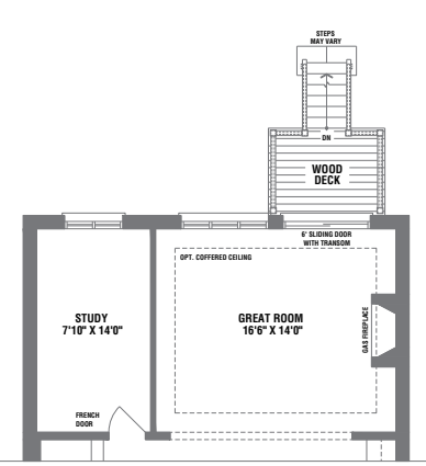
OPT. MAIN LEVEL W/ STUDY FOR LOT 5 & 37 ELEV. 'A', 'B' & 'C'
